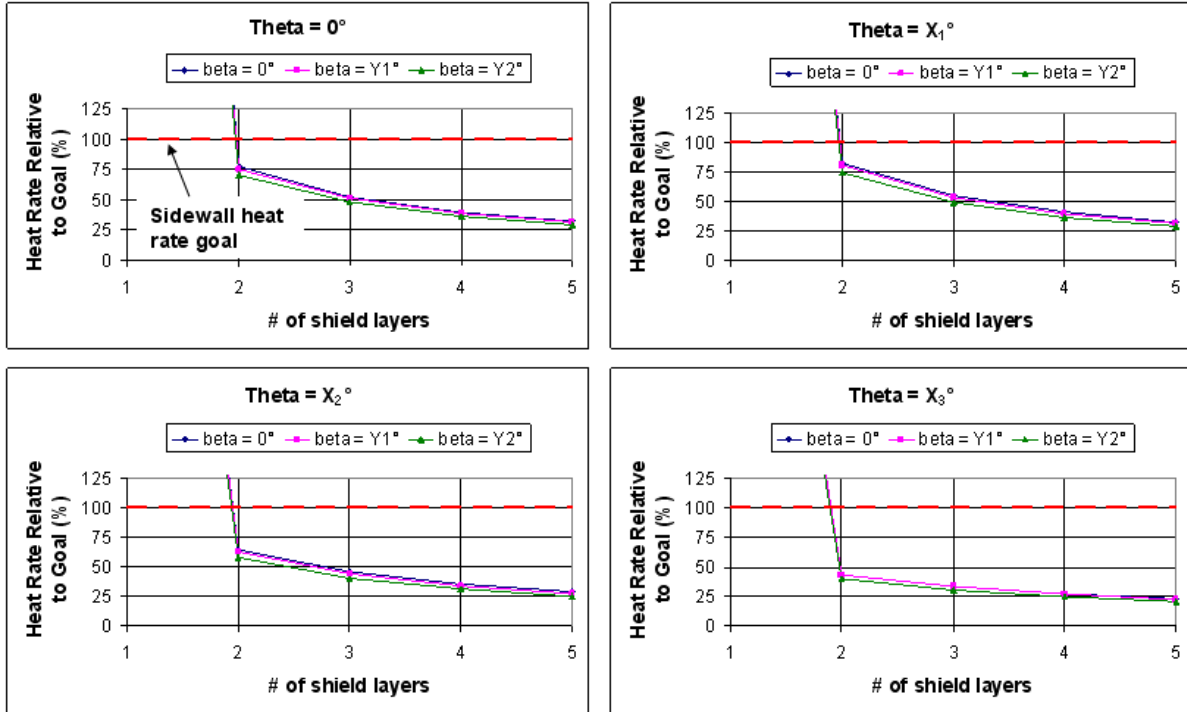
Figure 9: Predicted CSS Tank Heating Performance for Case 2 Shield Lay-up
