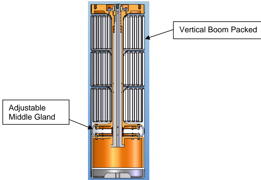
Figure 4: CSS Columnator Model, Packed Configuration
