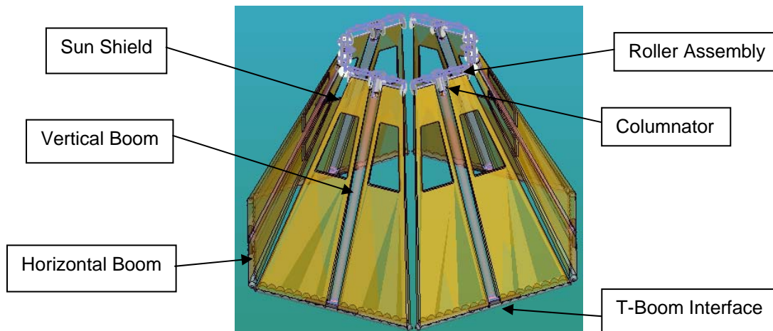
Figure 3: Centaur Sunshield Computer Model & Terminology
