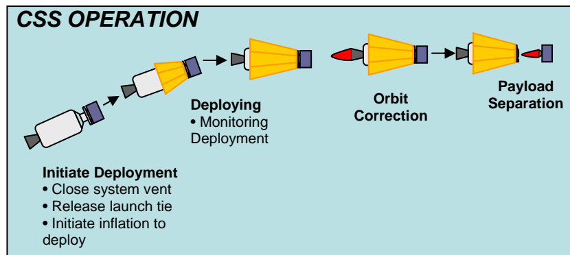
Figure 1: CSS Concept of Operations Schematic
