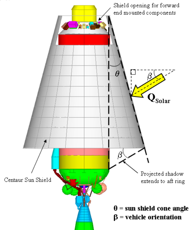
Figure 7: Centaur Sun Shield Design Parameters
