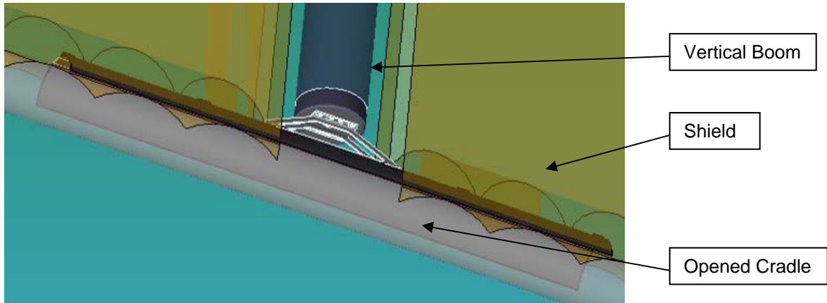
Figure 6: T-Boom Assembly Model
