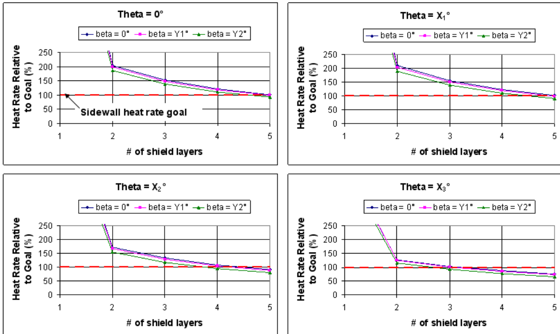
Figure 8: Predicted CSS Tank Heating Performance for Case 1 Shield Lay-up
