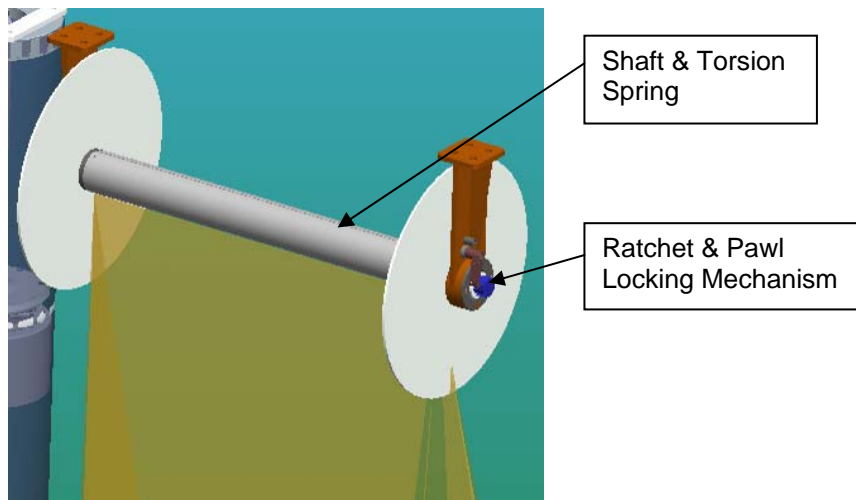
Figure 5: CSS Roller Assembly Model
